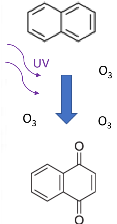
1,4-Naphtoquinone
